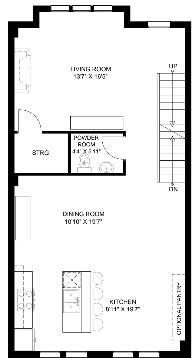
2ND FLOOR
