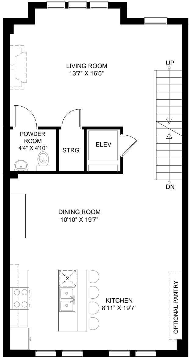
2ND FLOOR
